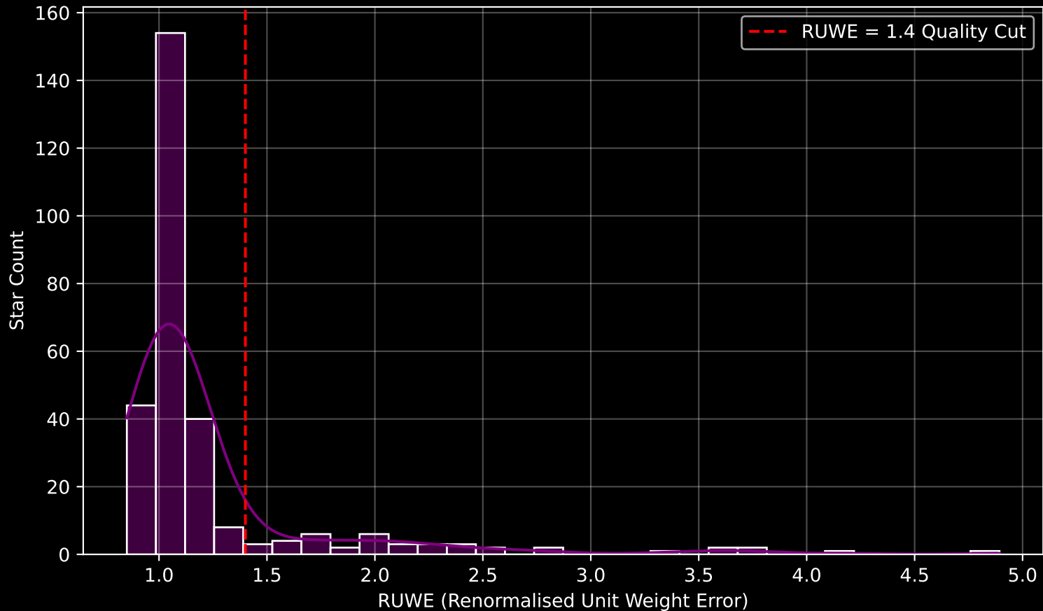
GALAH DR4 Field [6924] RUWE Distribution (n= 287)
