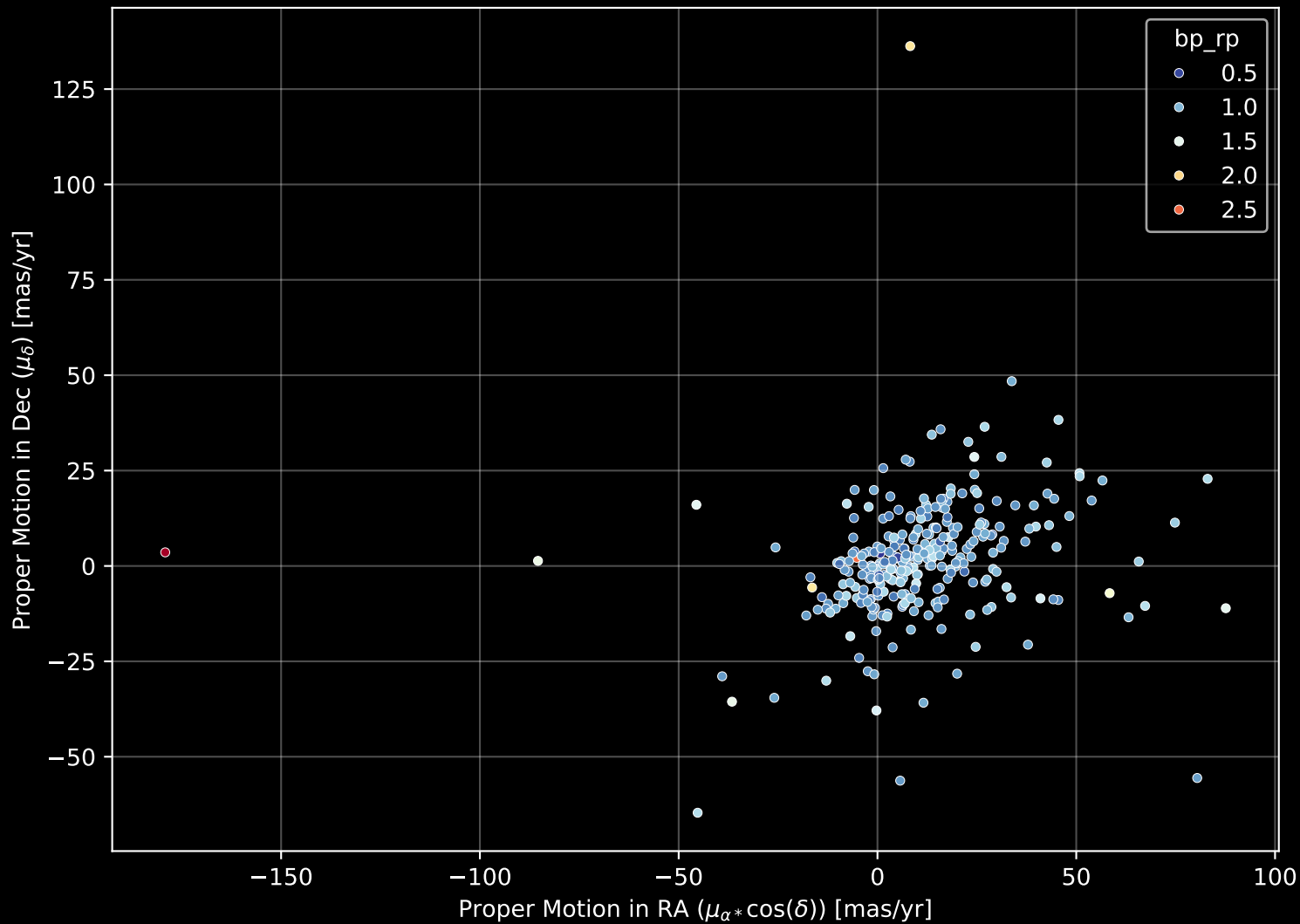
GALAH DR4 Field: [6924] Proper Motion Diagram (n= 299)
